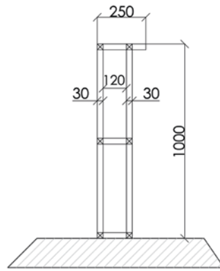
1 1/2 BAR FRAME SUPPORT
